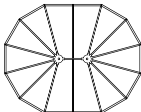
Gazebo walls 5000. 11' 6" x 14' 6". (14 walls of 36")
