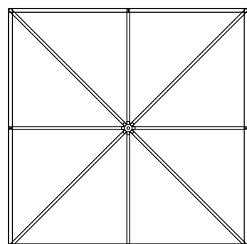
Gazebo walls 5000 10' 4" x 10' 4". (8 walls of 60")
