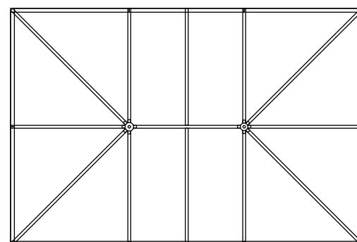
Gazebo walls 5000. 10' 4" x 15' 4". (10 walls of 60")
