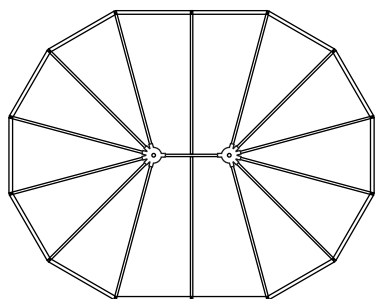
Gazebo walls 5000. 15' 3/8" x 19' 3/8". (14 walls of 48")
